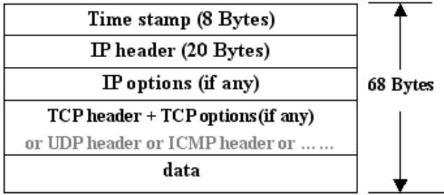
图1 Watcher 系统采集的原始数据格式 Fig.1 The format of raw data collected by Watcher system
